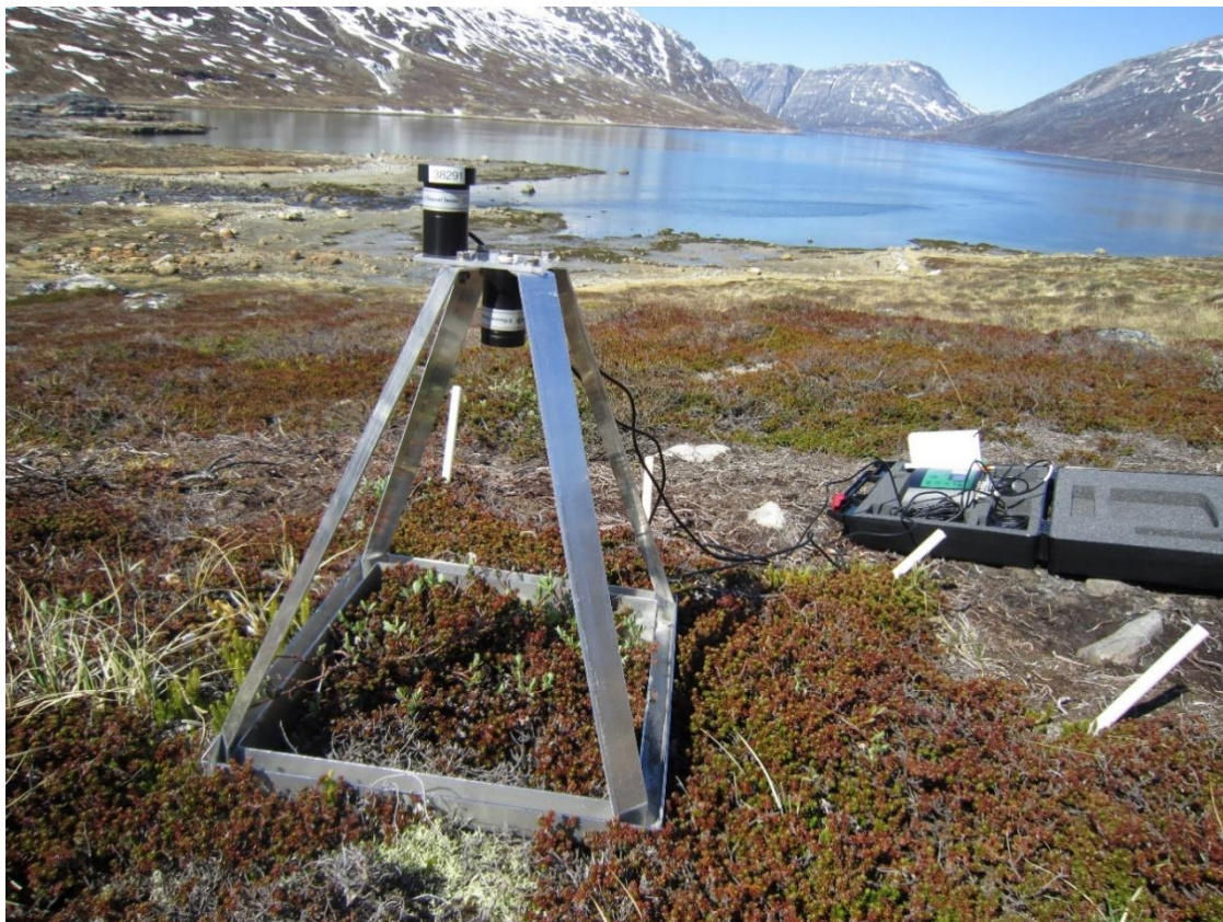
Figure 19. The light sensors attached to a plexiglas plate with 4 legs positioned in each of the corners of the flux plot metal frame. Notice the light sensor with the diffuser marked 38291 is facing upwards while the sensor without a diffuser (marked 38294) is facing downwards.
