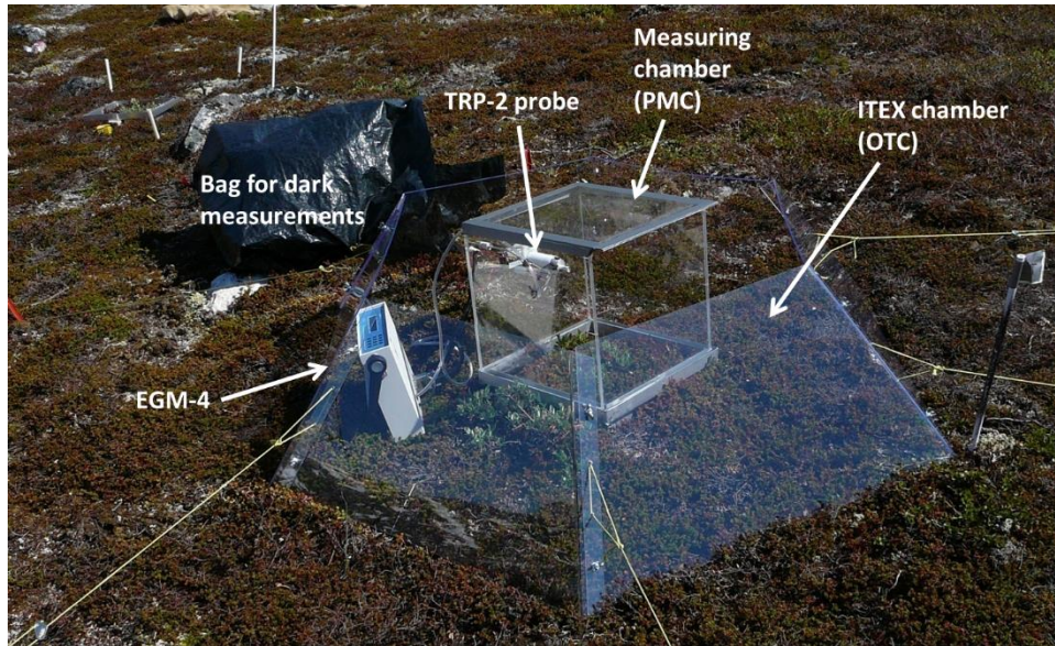
Figure 23. Measurement of CO 2 flux in an ITEX-hexagon open-top chamber with a measuring chamber (PMC) fitted with a TRP-2 probe connected to the EGM4. This setup resembles the “old” instrument and probe, though the setup with the new EGM5 and TRP-3 probe is similar. The black plastic bag is used for dark (respiration) measurements.
