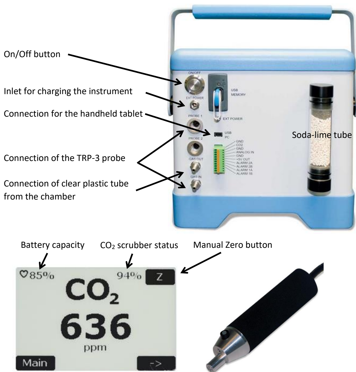
Figure 22. Top: The back of the EGM-5 instrument used for measuring CO 2 concentrations. Bottom, left: The touch display at the top of the EGM-5. Bottom, right: The TRP-3 temperature/PAR sensor.
