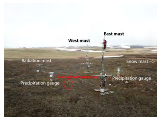
Figure 39: The Climate station includes two almost identical equipped masts. East and West, a separate radiation mast, two separate precipitation gauges and a snow mast (outside the photo). The Zackenberg station is in the background.
