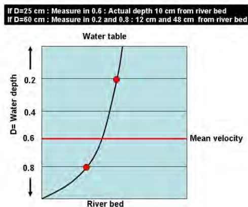
Figure 52: Standard velocity profile in the river and an example of measuring velocity at two different water depths.
