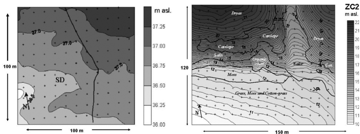
Figure 32: Surface topography/elevation at the two CALM-sites and borders between main vegetation communities in ZC-2.
