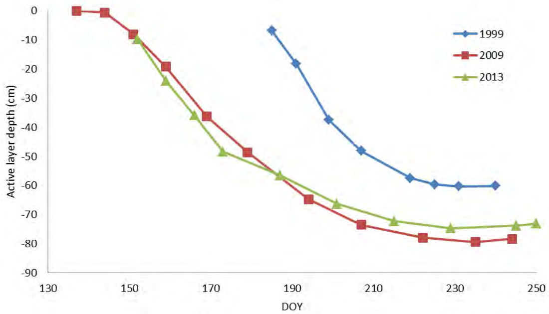
Figure 29: Thaw depth progression in ZEROCALM-1 in 1999, 2009 and 2013.
