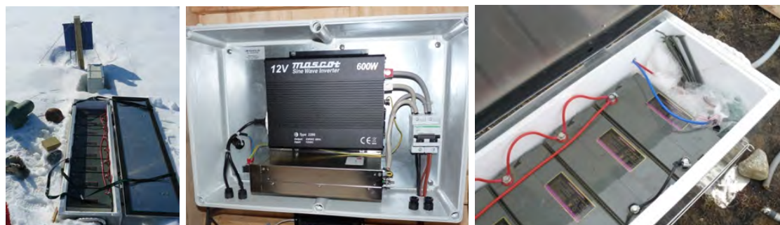
Figure 76: The battery box (left). A look into the transformer box, inside the hut (mid). Power cable from the instrument box enters the battery box in the southern end –the red and blue cable are connected to plus and minus on the last battery in the row.
