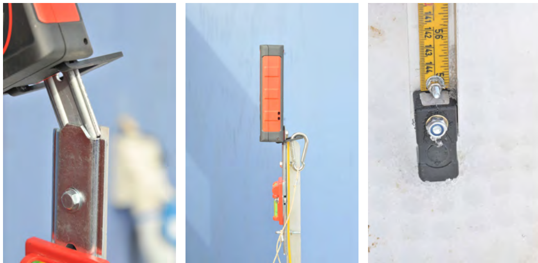
Figure 48: Correct mounting of range finder on pole with ruler (two leftmost photos) and placement of pole foot on a point directly under the hoist trolley (right photo).
