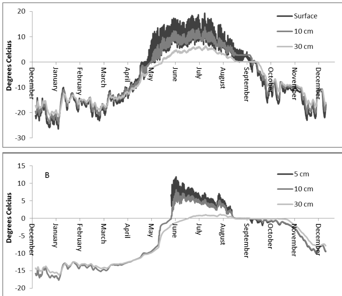
Figure 34: Seasonal variation from 2011 in soil temperatures under A) dry heath vegetation, dominated by Dryas integrifolia/octopetala and B) wet continuous fen, dominated by sedges. Notice different Y-axis.
