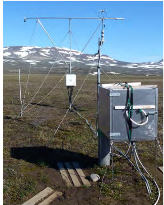
Figure 8: MM1 with energy balance mast, behind eddy covariance tower and enclosure instruments.
