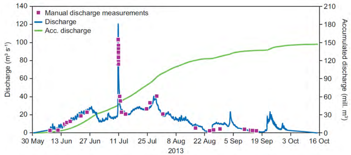
Figure 43: A typical season's discharge of Zackenberg river with manual discharge measurements (purple squares), the derived discharge time series (blue) and the accumulated discharge (green line).
