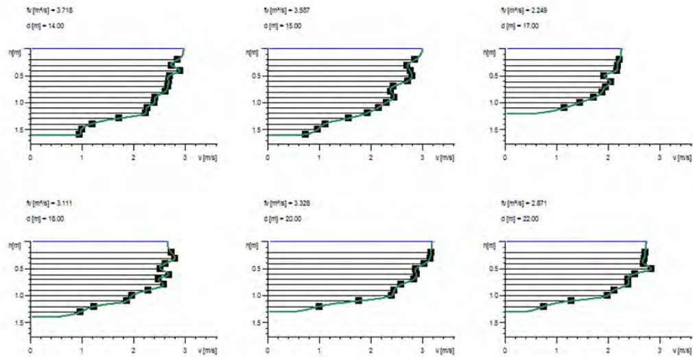
Figure 41: Example of flow velocity profiles at Zackenberg river on 16.08.2014. Note, that not all profiles follow a perfect logarithmic curve.
