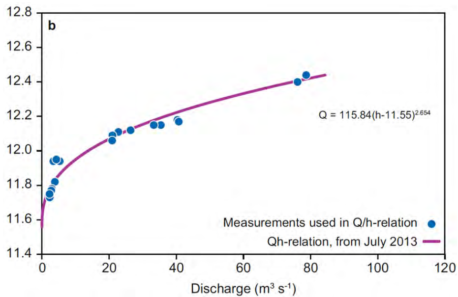
Figure 42: The Q/h relation for Zackenberg river for late 2013 with manual measurements (blue dots) and the derived relation (purple line). A new one had to be established after the GLOF from July 2013.
