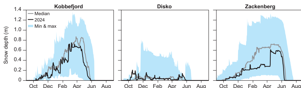
Figure 2. Snow depth measurements in 2024 (black lines) compared to min and max for the historical record (shaded area) and the median (grey line). Snow is a key parameter in Arctic ecosystem functioning. Several different methods are in use to get information on spatial distribution and temporal patterns in snow cover, across the three GEM sites. Methods include time-lapse photography, transect surveys, snow density measurements and, as shown here, long-term point-based monitoring of snow depth. Data used in the figure: Kobbefjord: 2008–2024, Disko: 2012–2024 and Zackenberg: 1997–2024.
