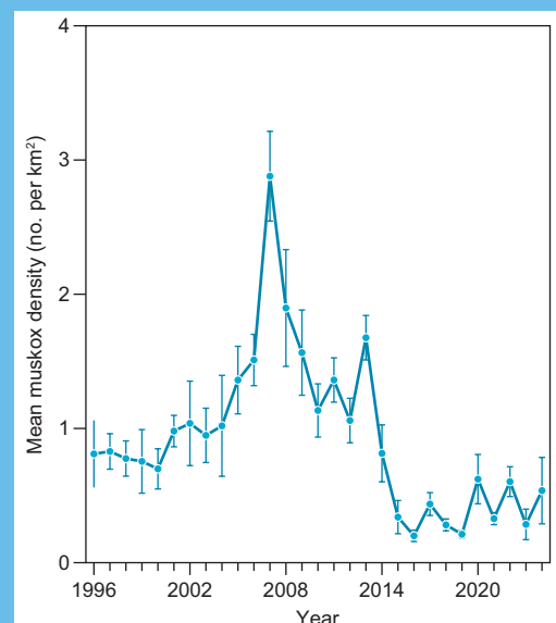
Figure 3. Inter-annual variation in muskox population dynamics (July and August) at Zackenberg 1996-2024.
