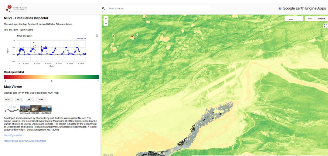
Figure 4. Example of GEMNDVI_Sentinel2 web application. Users can click on the map to extract NDVI time series and visualize NDVI images for selected dates.
