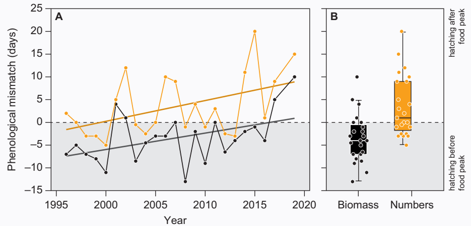
Figure 2. Mismatch between Sanderling median hatch dates and the date when 50% of cumulative arthropod abundance (orange) or cumulative arthropod biomass (black) was sampled in pitfalls in Zackenberg (1996–2019, excluding 2018). Positive values indicate that the median hatch date occurred after the 50% date in arthropod abundance or biomass. Fitted linear models are shown as solid straight lines. Boxplots summarize the spread in the data, where horizontal white bars indicate the median, the box depicts the interquartile range and whiskers represent 1.5 times the interquartile range from the upper/lower quartile. For visual clarity we applied a horizontal jitter to the raw data depicted in the boxplots.
