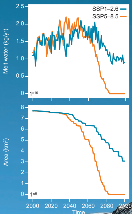
Figure 2. Chamberlin glacier on Lyngmarks-bræen at the Disko site. Top panel side shows projected melt from the glacier, bottom panel shows projected glacier area.
