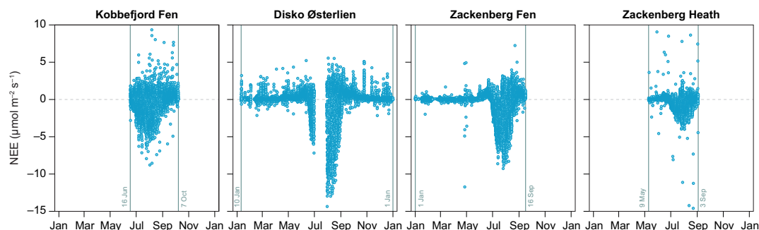
Figure 1. The Half-hourly Net Ecosystem \text{CO}_2 Exchange (NEE) is measured at the GEM/ICOS eddy covariance (EC) stations located at Kobbefjord Fen, Disko Østerlien, Zackenberg Fen, and Zackenberg Heath. Negative values indicate a net ecosystem sink of \text{CO}_2 , while positive values indicate a \text{CO}_2 source. Disko Østerlien is the only station connected to grid power, enabling year-round operation. Due to a logging failure in the anemometer no fluxes are presented from the Disko site in July. Zackenberg Fen operates on a reliable autonomous off-grid power system during the winter, currently undergoing testing. Kobbefjord Fen and Zackenberg Heath are restricted to operation only when the stations are accessible, affecting data coverage throughout the year (refer to the figure for start and end dates of operation). The range of fluxes varies considerably among ecosystems, with the smallest net \text{CO}_2 sink observed at the dry Zackenberg Heath.
