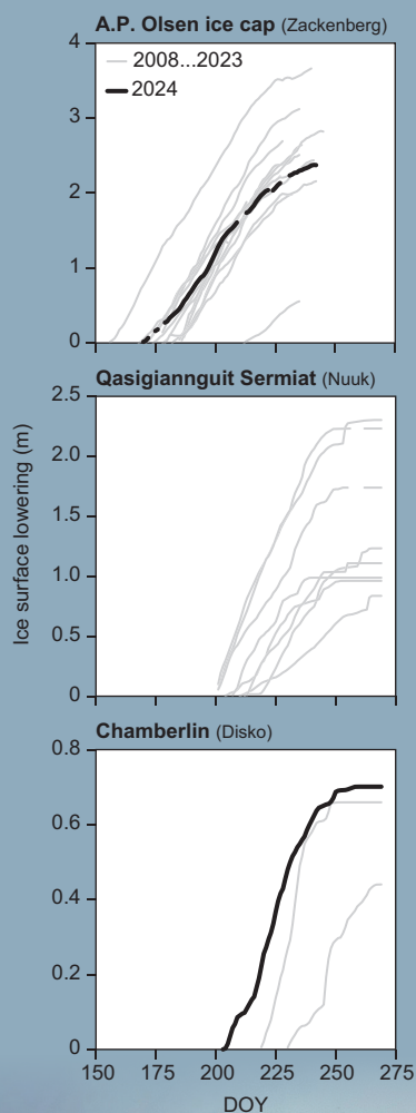
Figure 1. Ice surface lowering, directly convertible to ice melt, from GlacioBasis automatic ablation and weather stations in the ablation zone of the monitored glaciers at the three GEM sites in 2024 (black) vs. earlier years (gray).
