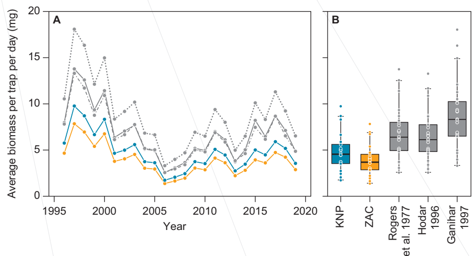
Figure 1. Estimates of average biomass per pitfall trap per day at Zackenberg (1996–2019), calculated based on regressions from five different sources. Data depicted in blue are calculated using family-level length-biomass regressions for Knipovich (KNP) and data in orange using family-level regressions for Zackenberg (ZAC). Data depicted in grey are calculated using order-level regressions extracted from literature, where the solid grey line is based on regressions from Rogers et al. (1977; Ann. Entomol. Soc. Am. 70: 51–53), the dashed grey lines on regressions from Hódar (1997; Misc. Zool. 20: 1–10) and the dotted grey line on regressions from Ganihar (1997; J. Biosci. 22: 219–224). Boxplots summarize the spread in the data, where horizontal white bars indicate the median, the box depicts the interquartile range and whiskers represent 1.5 times the interquartile range from the upper/lower quartile.
