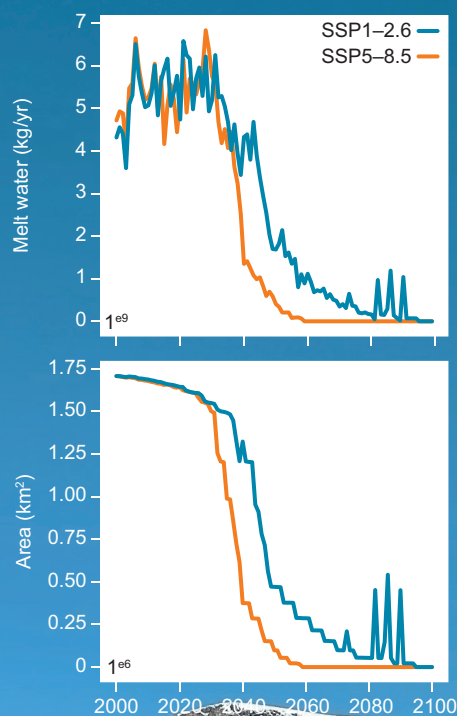
Figure 1. Qassinnguit Sermiat at the Kobbe-fjord site near Nuuk. Top panel shows projected melt from the glacier, bottom panel shows projected glacier area.
