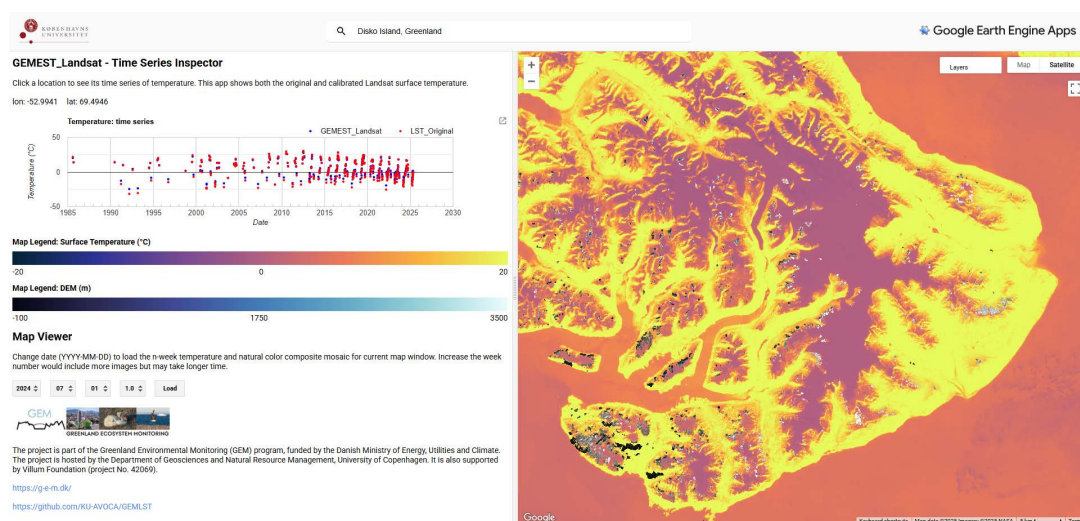
Figure 3. Web application of Land-sat-generated LST. Users can extract time series of surface temperature data by clicking on the map. The map viewer allows users to visualize the surface temperature image at given dates.
