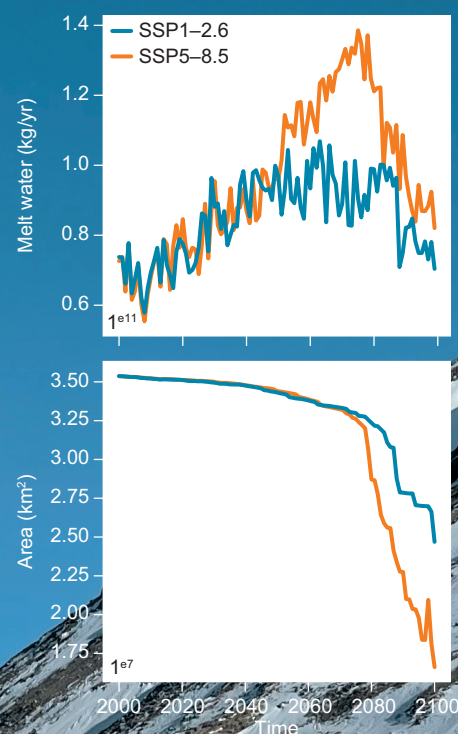
Figure 3. The monitored east flowing outlet of A.P. Olsen Ice Cap at the Zackenberg site. Top panel side shows projected melt from the glacier, bottom panel shows projected glacier area.
